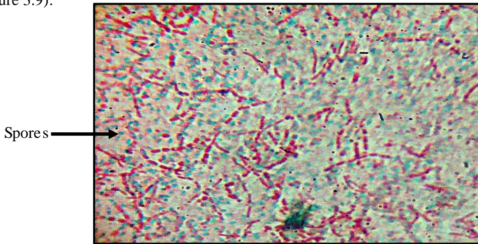
Figure 3.9: Appearance of isolate 14 after spore staining under the microscope. The spores are stained green whereas the bacterial cells are stained red
