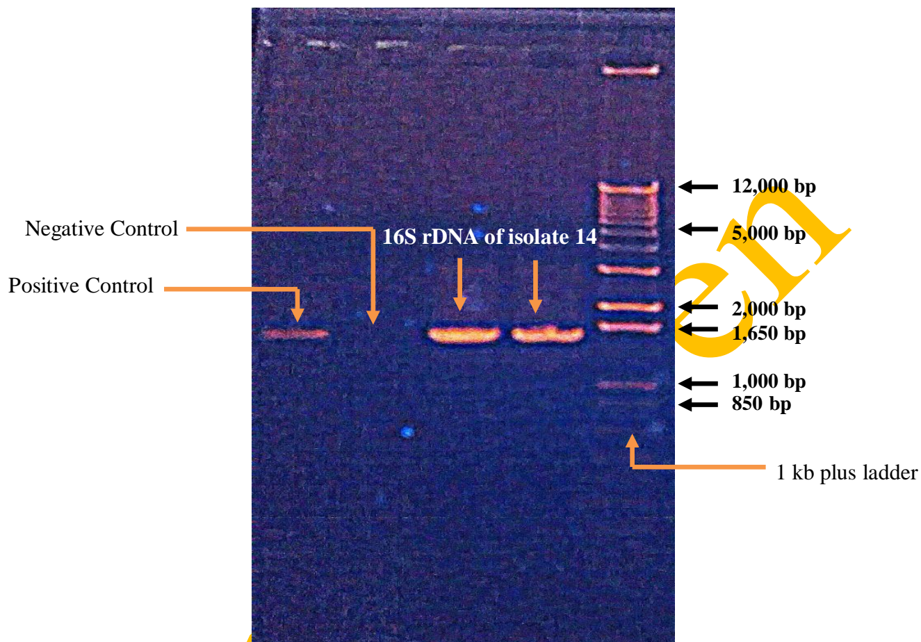
Figure 3.12: Visible DNA bands over UV illuminator on 1% agarose gel after electrophoresis. It can be seen that the 16S rDNA bands of isolate 14 which migrated along the lanes of wells 3 and 4 are slightly lower than 1,650 bp when compared to the ladder which migrated along the lane of well 5. Lane 1 indicates the DNA band of positive control and lane 4 shows that no band can be seen for the negative control.
